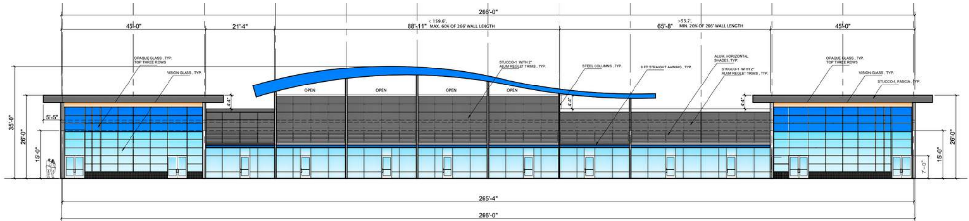
NORTH ELEVATION BUILDING-1
